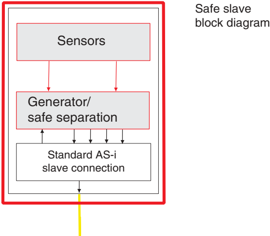
Figure 12.8: Block diagram of safe slave with two-channel safety component
