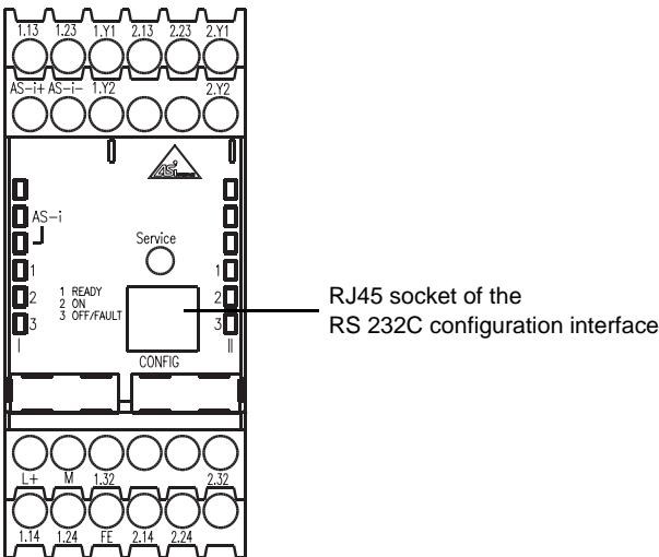
Figure 7.2: Location of the RS 232C configuration interface
