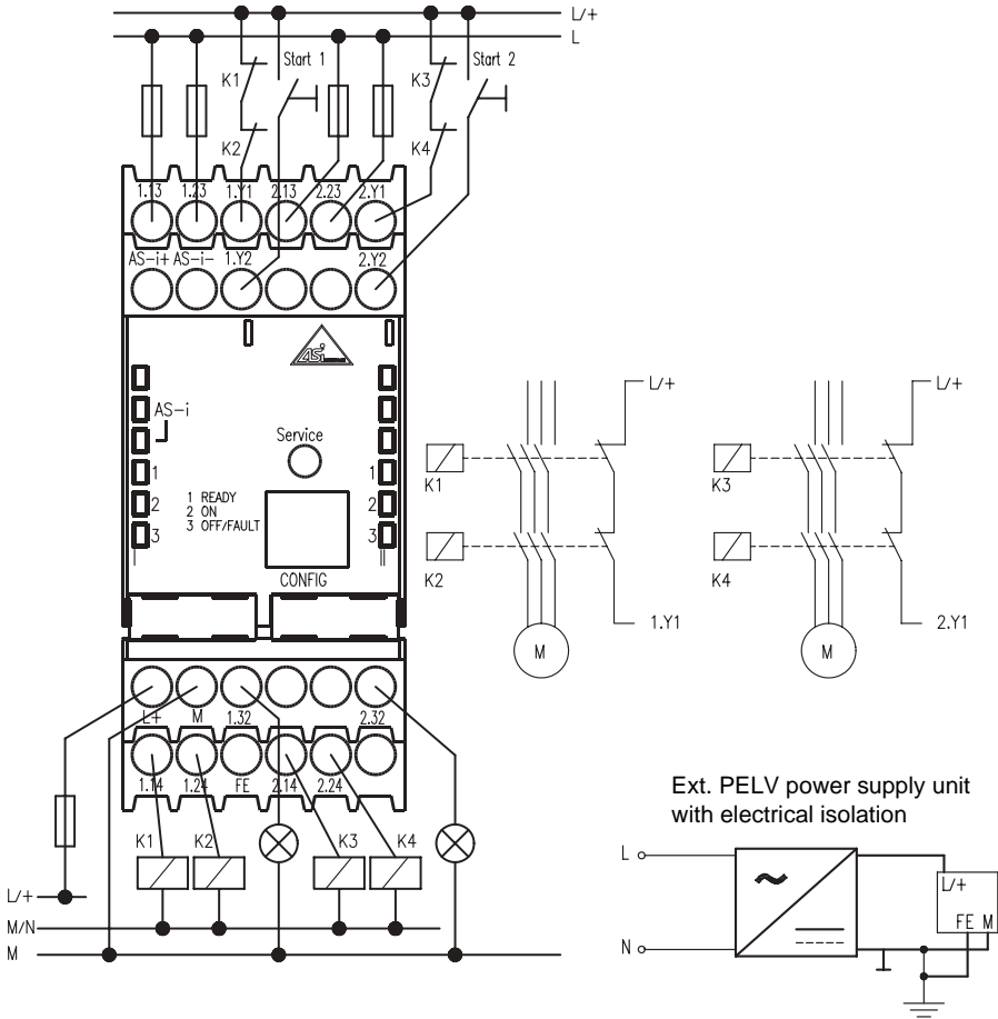
Figure 6.2: Connection overview of AS-interface safety monitor BW1763 and BW1765
