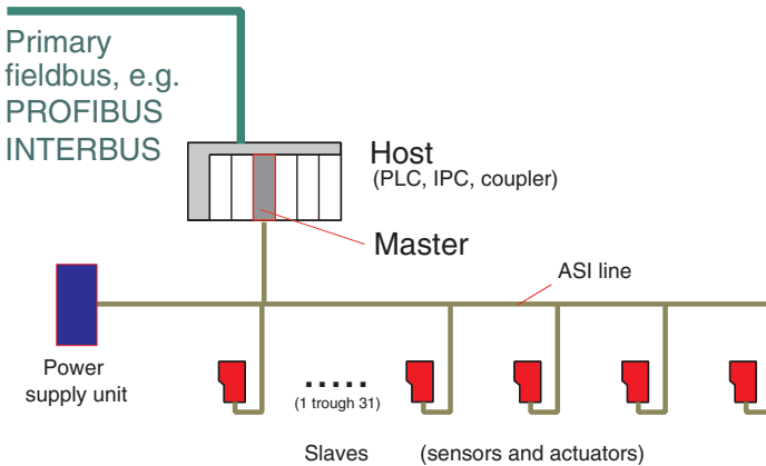
Figure 12.1: AS-interface system overview
