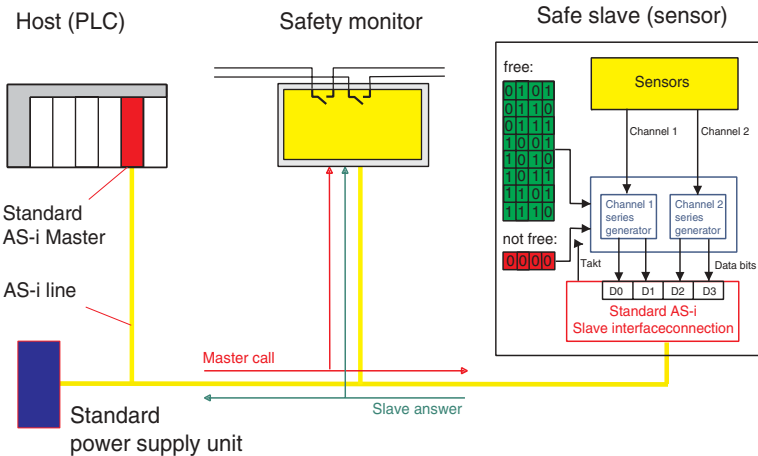
Figure 12.3: Safe data exchange
