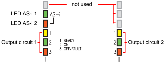
Figure 8.1: Overview of device LEDs
