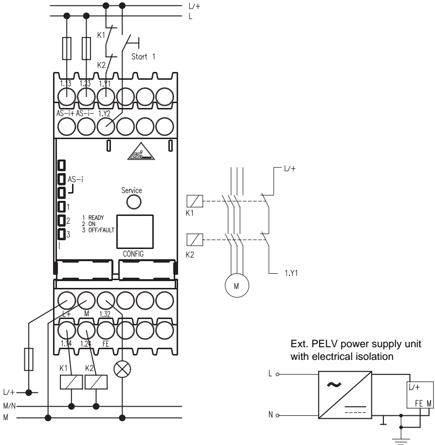
Figure 5.2: Connection overview of AS-interface safety monitor BW1762 and BW1764
