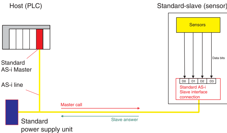
Figure 12.2: Data exchange in standard operation
