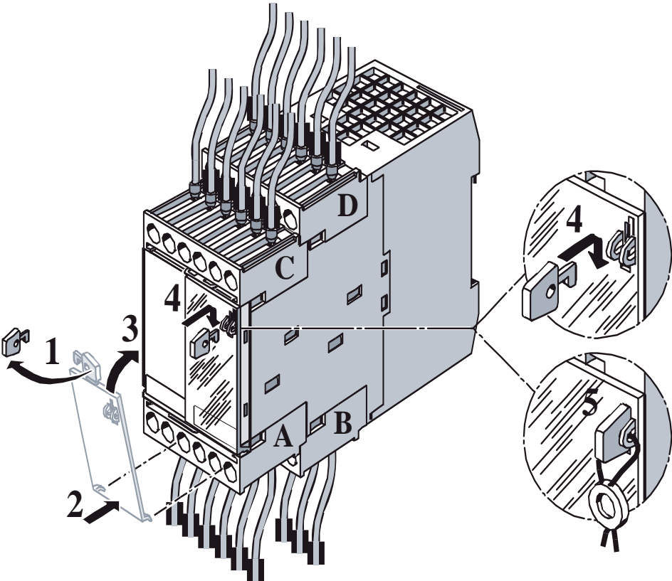
Figure 4.4: Mounting accessories for sealing the device
