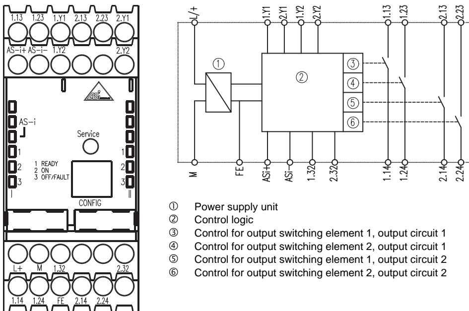
Figure 6.1: Terminal arrangement / block diagram of AS-interface safety monitor BW1763 and BW1765
