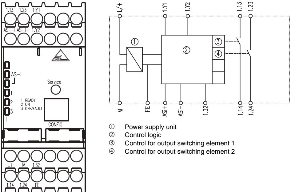
Figure 5.1: Terminal arrangement / block diagram of AS-interface safety monitor BW1762 and BW1764
