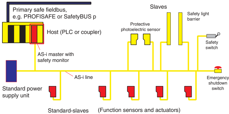
Figure 12.6: System design with safe host
