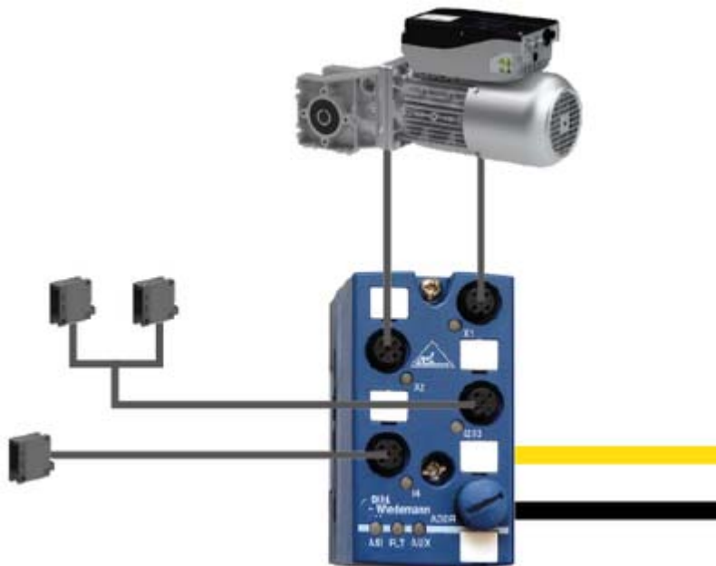
Fig. The AS-i 3.0 motor module for Lenze Smart Motors ( BWU3115 ) can control up to 5 speeds.
