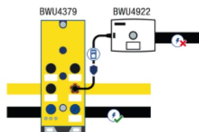
Safety-switched AUX branch in the field
