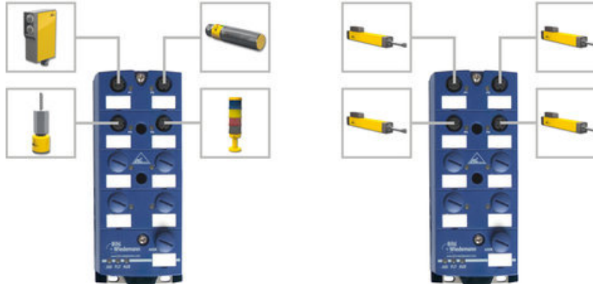
Fig.: AS-i/IO-Link Modules, IO-Link Master – available with 4 IO-Link Ports Class A ( BWU2853 ) or Class B ( BWU3020 ) – perfect compatibility with the IO-Link products from many manufacturers
