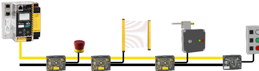
Fig.2: Active distributors: Make any sensors and actuators bus-capable
