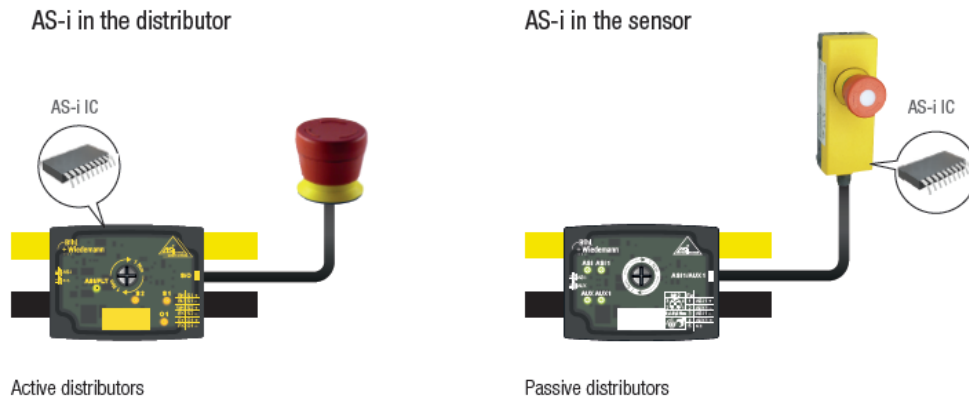
Fig.1: Active distributors, AS-i in the distributor (left); Passive distributors, AS-i in the sensor (right)
