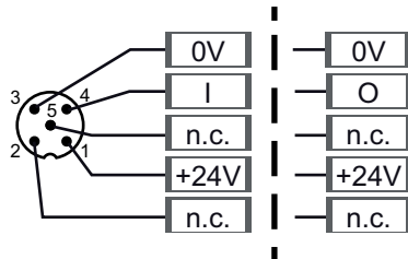
Single-wiring
