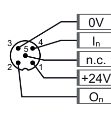
Mixed-wiring
